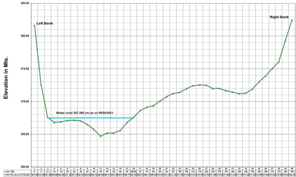
Pre Monsoon X-Section of Rupaligad GDS Site at 250 m D/S of Existing Centre Gauge Line as on 08.04.2021
