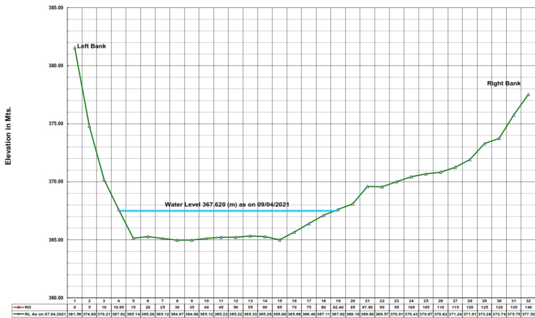
Pre Monsoon X-Section of Rupaligad GDS Site at 450 m D/S of Existing Centre Gauge Line as on 09.04.2021
