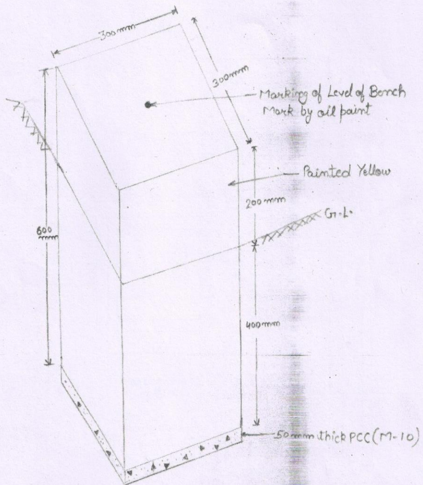
R.C.C. (M-15) Bench Mark (300x300x600mm)
