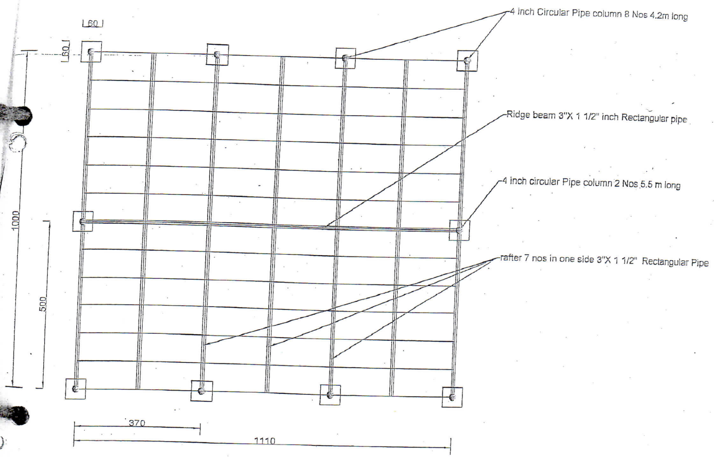
DETAILS OF TRUSS
